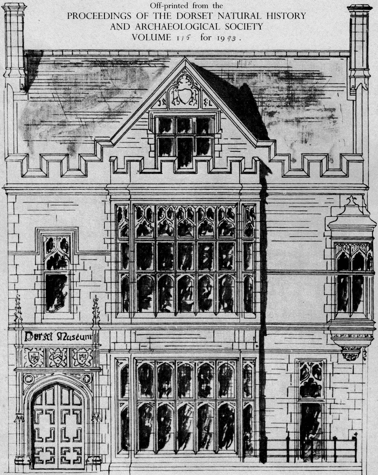
Drawing for the new Dorset County Museum, 1880, by the architect G. R. Crickmay.
